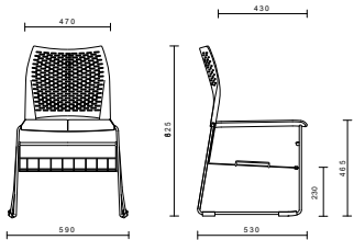
MAGAZINE BASKET
