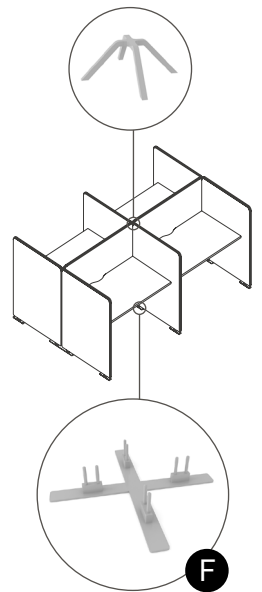
Metal X-shaped leg and fixator
