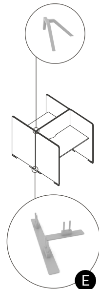
Metal T-shaped leg and fixator for the side screen
