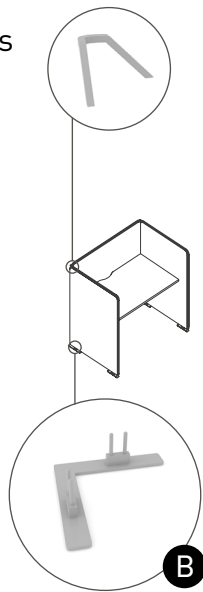
Metal L-shaped leg and left fixator
