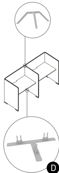
Metal T-shaped leg and fixator for the front screen
