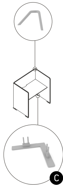
Metal L-shaped leg and right fixator
